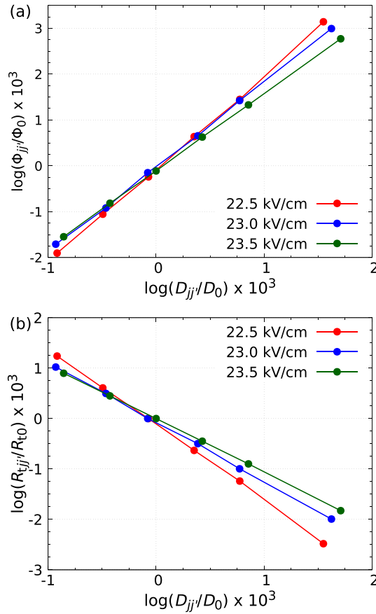
Figure 7. (a) Phase integrals \Phi_{jj'} and (b) inner turning points R_{tjj'} for different spin states j as a function of dipole length D_{jj'} , for three different electric fields in the shielding region. All quantities are expressed as ratios to their spin-free values. The slopes of the plots show that, at each field, \Phi_{jj'} scales approximately as D_{jj'}^2 and R_{tjj'} scales approximately as D_{jj'}^{-1} .
