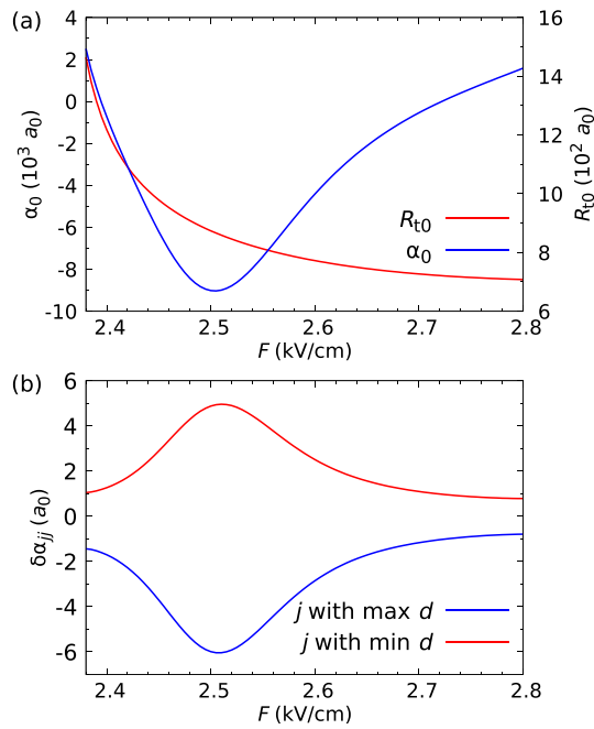
Figure 8. Predicting spin-dependent changes in scattering length for NaCs from the model. (a) Spin-free turning point R_{t0} and real part of scattering length \alpha_0 for NaCs at fields where shielding is effective; (b) real parts of \alpha_{ij} from equation (7), including the effects of spin, shown as differences \delta\alpha_{ij} from spin-free values. Results are shown for spin states j with maximum and minimum values of d_j and span the range of possible values of \delta\alpha_{ij} .
