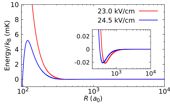
Figure 2. Effective potentials (adiabats) for spin-free CaF at the threshold (\tilde{n}, m_n) = (1, 0) + (1, 0) for fields of 23 and 24.5 kV cm -1 . The differences between the adiabats at different fields allow tuning of the scattering length. The inset shows an expanded view of the long-range potential well.
