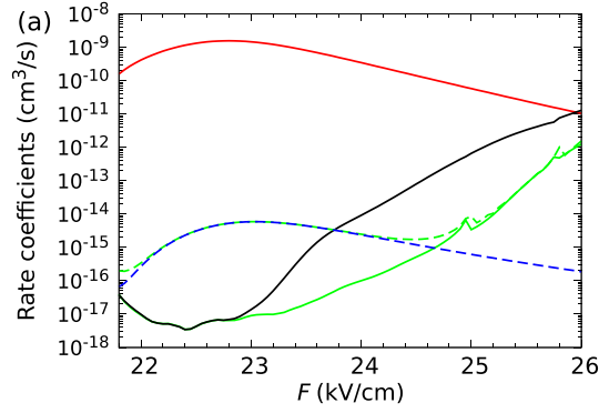
Figure 3. Collision rate coefficients for CaF. Solid lines show spin-free rate coefficients for elastic scattering (red), inelastic scattering (green) and short-range loss (black) at collision energy E_{\text{coll}} = 10 \text{ nK} \times k_B , over the range of electric fields F where shielding is effective. The corresponding results including spin, for molecules in the initial pair state (g, m_g) = (1, 1) + (1, 1) , are shown as dashed lines. The resulting curves for elastic scattering and short-range loss lie underneath the spin-free ones. The dashed blue line shows the contribution from the 1-molecule inelastic transition to (1, 0) + (1, 1) . The calculations including spin use the spin-N206-L6 basis set described in appendix B.
