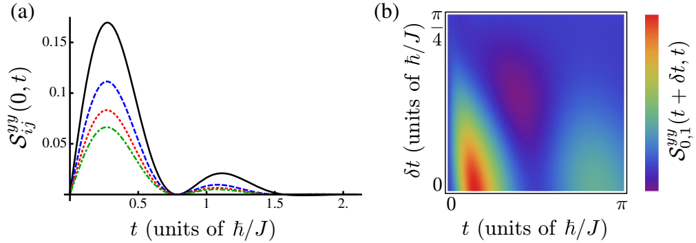
Figure 5. Connected dynamical correlation function \mathcal{S}_{ij}^{yy}(t_1, t_2) = S_{ij}^{yy}(t_1, t_2) - S_i^y(t_1)S_j^y(t_2) for a 100 site 1D chain with \zeta = 1 and nearest-neighbor coupling J . In (a) we plot \mathcal{S}_{i,i+r}^{yy}(0, t) for i = 50 and r = \{2, 3, 4, 5\} (from top to bottom). In (b) we plot \mathcal{S}_{i,i+1}^{yy}(t, t + \delta t) (again for i = 50 ) as a function of t and \delta t . In both plots the initial state consists of all spins pointing in the +x direction ( \theta = \pi/2 and \phi = 0 ).
