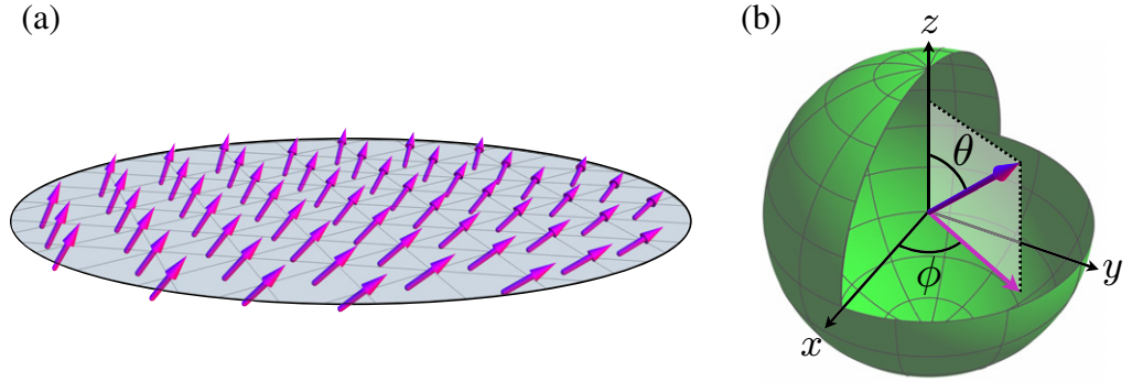
Figure 1. The only restriction on the initial state is that it be unentangled (i.e. a product state over the various sites in the spin model). For example, one can imagine (a) an initial state with some slow spatial variations in the spin angles due to inhomogeneities in the pulse strength of a Ramsey-type experiment. The notation used to characterize the state of any one spin is shown on the Bloch sphere in (b).
