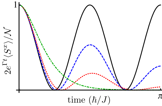
Figure 7. Here we plot the transverse spin length S^x as a function of time in a 1D nearest-neighbor Ising model, with \{\Gamma_{\text{el}}, \Gamma_{\text{ud}}, \Gamma_{\text{du}}\} = \{0, \Gamma, \Gamma\} . Different curves correspond different values of \Gamma between 0 (undamped) and \Gamma_c (critically damped): \Gamma = 0 (black solid line), \Gamma = \Gamma_c/8 (blue dashed line), \Gamma = \Gamma_c/4 (red dotted line) and \Gamma = \Gamma_c (green dot-dashed line).
