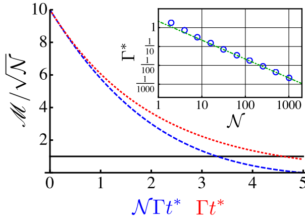
Figure 11. Metrological gain over the standard quantum limit ( \mathcal{M}/\sqrt{N} ) of N=100 spins evolved under the OAT Hamiltonian to a time t^* (where a GHZ state exists in the absence of decoherence). We plot \mathcal{M} as a function of decoherence rates for pure dephasing ( \{\Gamma_{\text{el}}, \Gamma_{\text{ud}}, \Gamma_{\text{du}}\} = \{\Gamma, 0, 0\} , red dotted line) and for spontaneous relaxation ( \{\Gamma_{\text{el}}, \Gamma_{\text{ud}}, \Gamma_{\text{du}}\} = \{0, \Gamma, 0\} , blue dashed line). Note the two curves are produced by rescaling the decoherence rates in different ways (in order to show them in the same plot); if the scaling were the same for both plots, \mathcal{M} would decay much more quickly for spontaneous relaxation than for dephasing. Inset: log-log plot of \Gamma^* , defined to be the decoherence rate for which \mathcal{M} has decreased to N/e , as a function of N (blue circles). The green dot-dashed line represents (up to a multiplicative constant) 1/N scaling.
