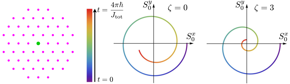
Figure 3. Trajectories of the Bloch vector S_0 projected into the xy plane, for all-to-all (left) and dipolar (right) couplings. Here j = 0 labels the central site (green dot in left panel) of a 55-site triangular lattice, and all spins are initialized at \{\theta_j, \phi_j\} = \{\pi/4, 0\} . In both cases we choose a nearest-neighbor coupling J , and scale the time by J_{\text{tot}} = \sum_{j \neq 0} J/(\mathbf{r}_j - \mathbf{r}_0)^\zeta . This rescaling of time is used so that different range interactions give rise to comparable precession rates. Note that at mean-field level the trajectory would close on itself. The inward spiral indicates the growth of quantum correlations and resultant decay of the spin length, and—in these rescaled time units—is more significant for shorter-range interactions.
