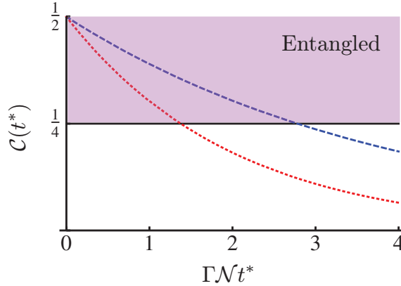
Figure 10. Here we plot \mathcal{C}(t^*) (a measure of the coherence of a GHZ state, described in the text) created in the presence of various types of decoherence: \{\Gamma_{\text{el}}, \Gamma_{\text{ud}}, \Gamma_{\text{du}}\} = \{\Gamma, 0, 0\} (dephasing, dashed blue line) and \{\Gamma_{\text{el}}, \Gamma_{\text{ud}}, \Gamma_{\text{du}}\} = \{0, \Gamma, 0\} (spontaneous relaxation, dotted red line). The region above the solid black line is guaranteed to have \mathcal{N} -particle GHZ type entanglement.
