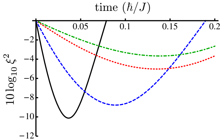
Figure 4. Optimal spin squeezing \xi as a function of time for a variety of power-law couplings J_{ij} = J/|\mathbf{r}_i - \mathbf{r}_j|^\zeta . The different curves correspond to: infinite ranged ( \zeta = 0 , black solid line), coulombic ( \zeta = 1 , blue dashed line), dipolar ( \zeta = 3 , red dotted line), and nearest neighbor ( \zeta = \infty , green dot-dashed line). For this calculation we take the spins to all point along the x -axis at t = 0 , and use 55 sites of a triangular lattice (the same as shown in figure 2).
