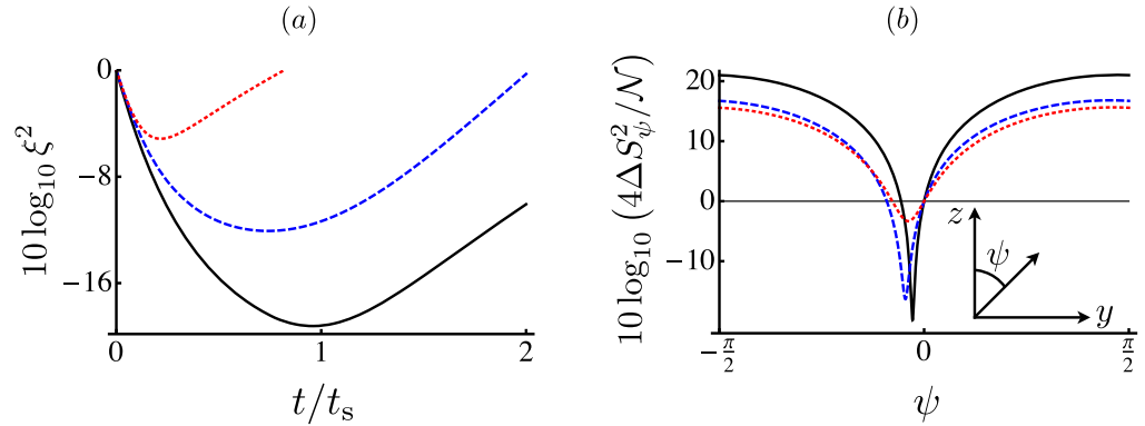
Figure 9. Spin squeezing \xi (in dB) of \mathcal{N} = 10^3 spins with no decoherence (black solid line), pure dephasing ( \{\Gamma_{\text{el}}, \Gamma_{\text{ud}}, \Gamma_{\text{du}}\} = \{\Gamma, 0, 0\} , blue dashed line), and equal amounts of spontaneous relaxation/excitation ( \{\Gamma_{\text{el}}, \Gamma_{\text{ud}}, \Gamma_{\text{du}}\} = \{0, \Gamma/2, \Gamma/2\} , red dotted line). In (a) we show the optimal squeezing (optimized over angle \psi ) as a function of time. In (b) we plot the normalized variance, evaluated at time t_s , as a function of the squeezing angle \psi . Note that at the angle of maximal squeezing ( \psi \approx 0 ), dephasing is much less detrimental than spontaneous relaxation/excitation, whereas both have a similar effect at the angle of maximal antisqueezing ( \psi \approx \pi/2 ). In all plots, we choose \Gamma = 1/t_s , with t_s = \hbar \mathcal{N}^{-2/3} (3^{1/6}/2J) being the time of optimal squeezing in the absence of decoherence.
