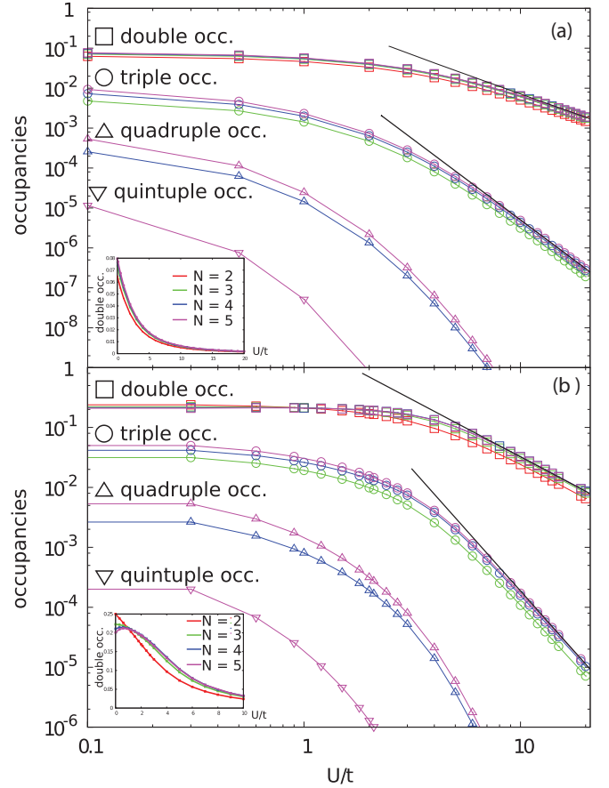
FIG. 8. (Color online) Site averaged double, triple, quadruple, and quintuple occupancies as a function of U/t for small systems at filling (a) n = 1/(2N) , and (b) n = 1/N . The system sizes in (a) are L = 24 for N = 2, 3, 4 , and L = 20 for N = 5 . The system sizes in (b) are L = 20 for N = 2, 4 , L = 21 for N = 3 , and L = 10 for N = 5 . The black straight lines are a guide to the eyes showing the power-law behavior. The insets show the double occupancy as a function of U/t for the different values of N .
