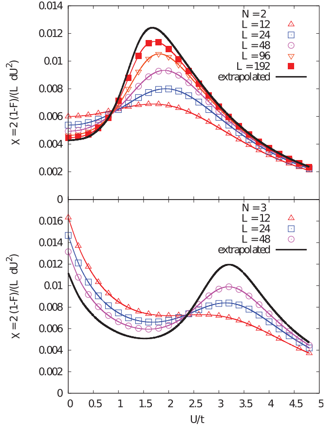
FIG. 5. (Color online) Fidelity susceptibility for different system sizes for N=2 and N=3 . The black continuous line shows the value after extrapolating to the thermodynamic limit using the system sizes shown.
