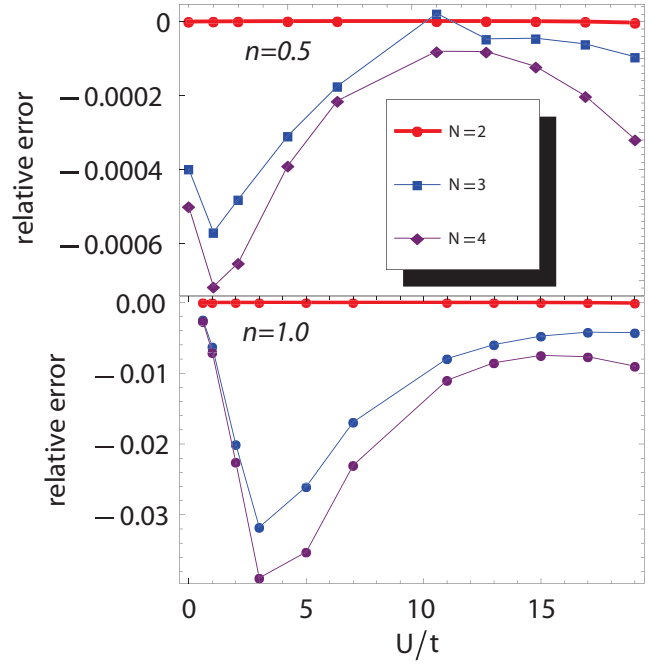
FIG. 2. (Color online) Relative error between DMRG and BA for N = 2, 3, 4 at densities n = 0.5 [ 1/(2N) filling, top] and at n = 1 [ 1/N filling, bottom].
