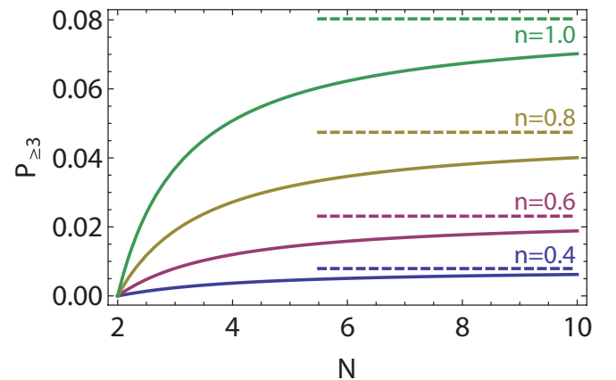
FIG. 3. (Color online) Triple or higher occupancy ( P_{\geq 3} ) vs N for various densities n .
