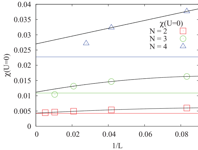
FIG. 4. (Color online) Finite size extrapolation of \chi(U=0) for N=2, 3, 4 . The horizontal lines show the exact values of Table I. For N=3 and N=4 we have not taken into account the results for the largest system sizes ( L=96 and L=36 , respectively) due to a discarded weight of similar order of magnitude as 1 - \mathcal{F}(U) . The black lines show a quadratic fit for N=2 and N=3 and a linear fit for N=4 .
