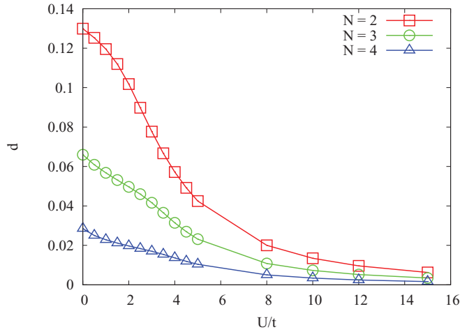
FIG. 10. (Color online) Distance d [Eq. (25)] between the spin correlation functions of the 1/N filled Hubbard and of the Heisenberg chains [Eqs. (7) and (6)] as a function of U/t for N \leq 4 .
