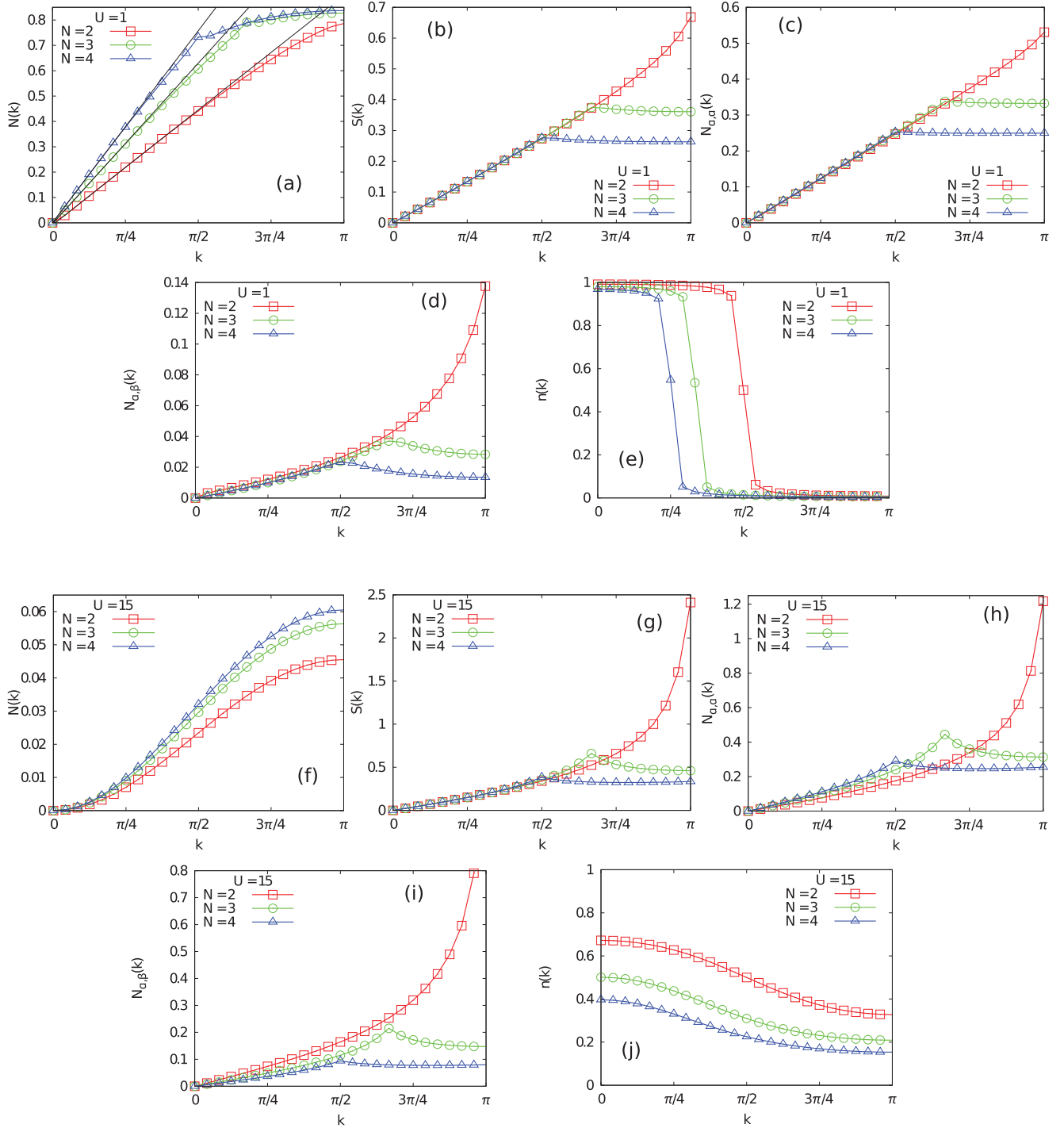
FIG. 12. (Color online) Structure factors of the various correlation functions Eqs. (7)–(11). (a) Charge structure factor [Eq. (10)] for U = t . (b) Spin structure factor [Eq. (7)] for U = t . (c) Structure factor N_{\alpha,\alpha}(k) [Eq. (8)] for U = t . (d) Structure factor N_{\alpha,\beta}(k) [Eq. (9)] for U = t . (e) Momentum distribution function [Eq. (11)] for U = t . (f)–(j): The same quantities, but for U = 15t .
