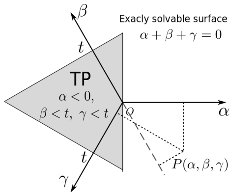
FIG. 1: Topological phase (TP) of the double wire system. The constraint \alpha + \beta + \gamma = 0 restricts the parameter space to the 2D plane drawn in this figure, where the coordinate (\alpha, \beta, \gamma) of an arbitrary point P is given by the projections from P to the \alpha, \beta, \gamma axes. The conditions \alpha < 0, \beta < t, \gamma < t , which guarantee \hat{H} to be positive definite, give a triangle region (shaded area) in this plane.
