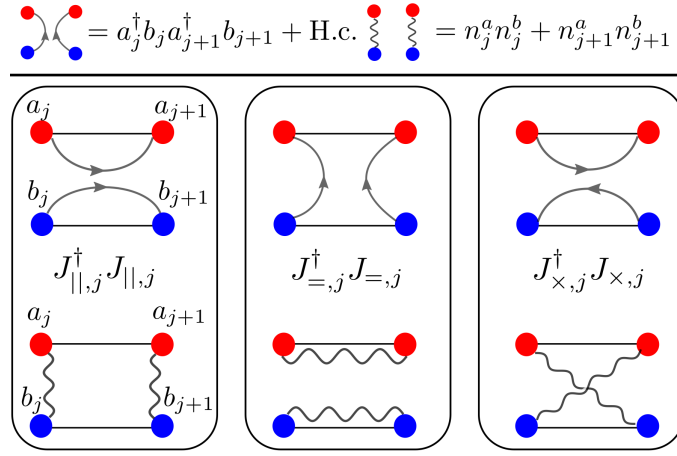
FIG. S1: Diagrammatic representation of interaction terms in the double wire parent Hamiltonian in Eq. (9). Double arrows represent pair hopping while wavy lines represent interactions.
